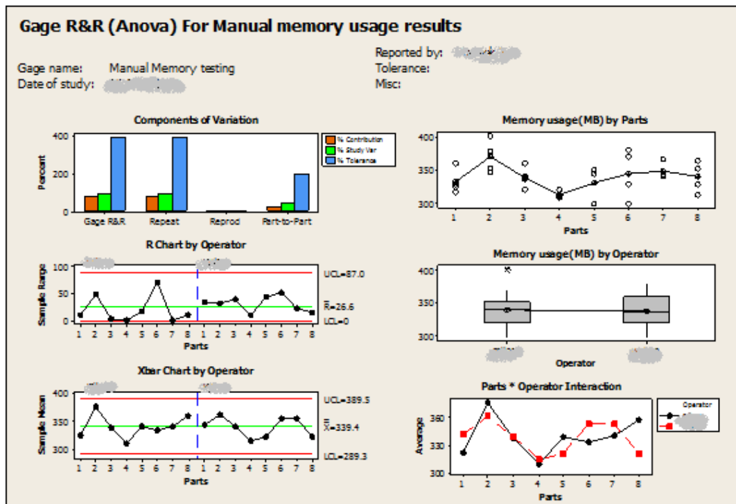
Figure 16: Gage R&R - Manual Process
