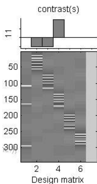
Figure 17. T-contrast
