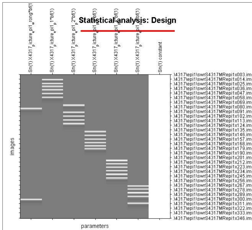
Figure 13. Design matrix
