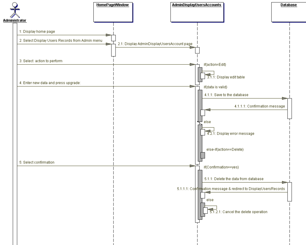
Figure 2-17 Sequence diagram of administrator viewing user records
