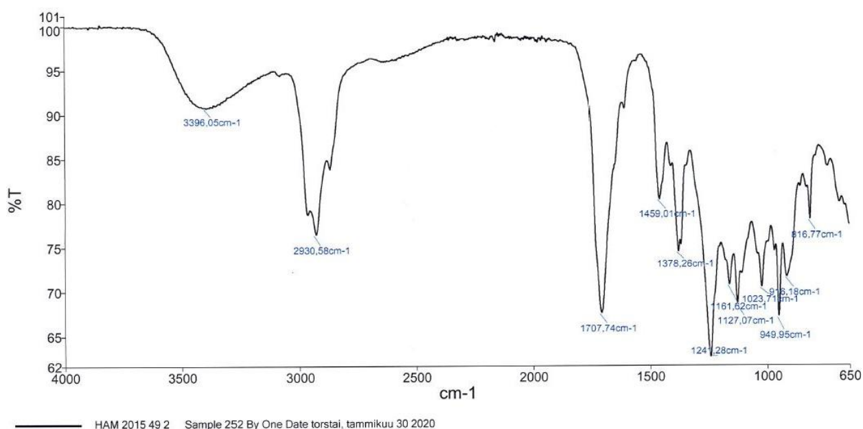
Figure 16. FTIR-spectrum from HAM varnish sample.
