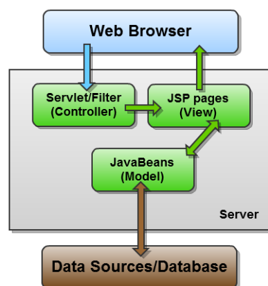
FIGURE 15: JSP layer separation
