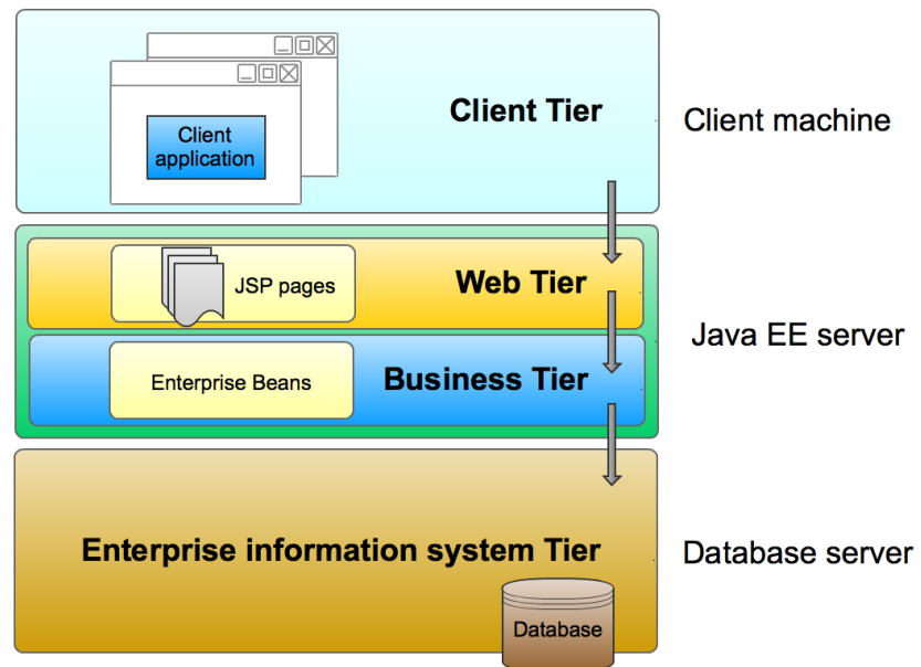
FIGURE 2: Multitiered applications
