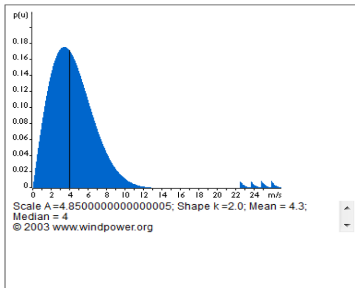
FIGURE 1. Weibull distribution
