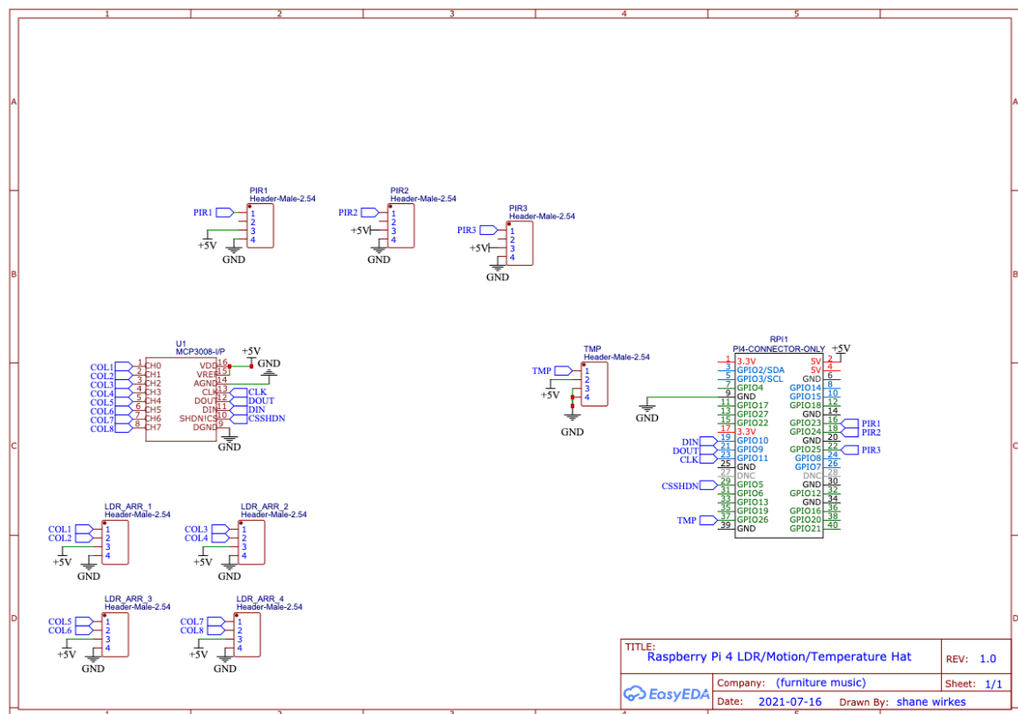
Figure 2. HAT Schematic.
