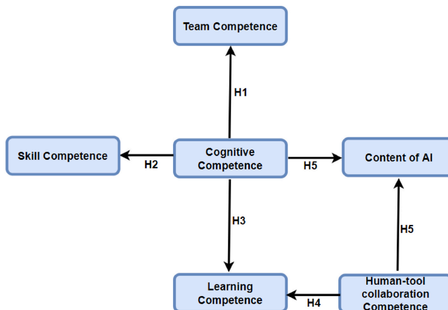
Fig. 2. Research model.
