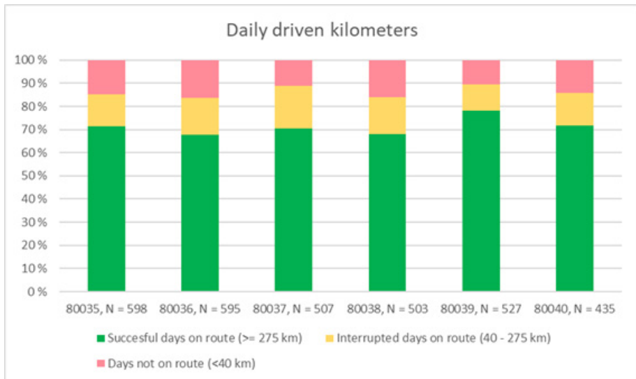
Figure 1. Classification of days according to kilometers driven by vehicle from October 2016 – November 2018
