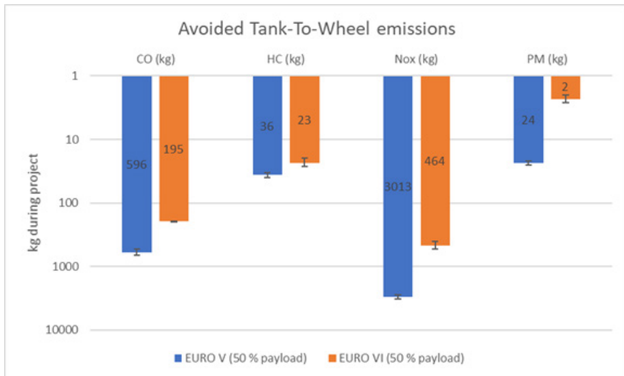
Figure 38. Avoided tank-to-wheel emissions, other emission components
