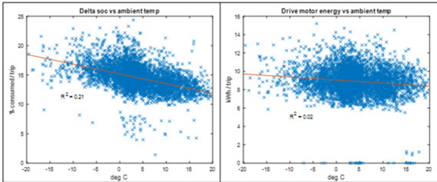
Figure 27. Delta SOC and driving energy vs ambient temperature
