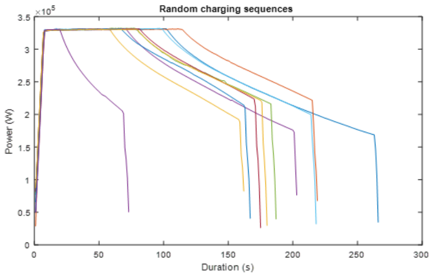
Figure 32. Random charging sequences measured from charger
