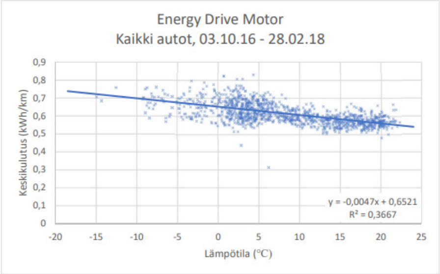
Figure 29. Average daily consumption of the drive motor (kWh / km) vs average daily temperature (° C) (Taavetinkangas 2018)
