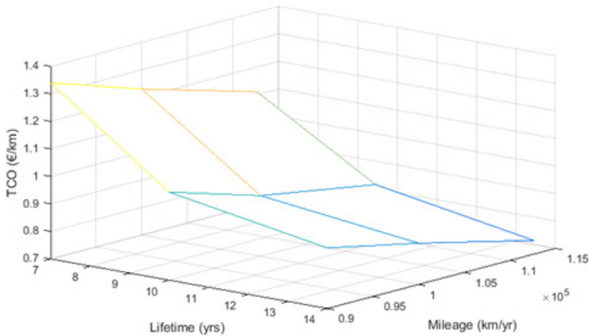
Figure 36. TCO as a function of yearly mileage and the vehicle lifetime in years. (Adapted from Lankila 2017)
