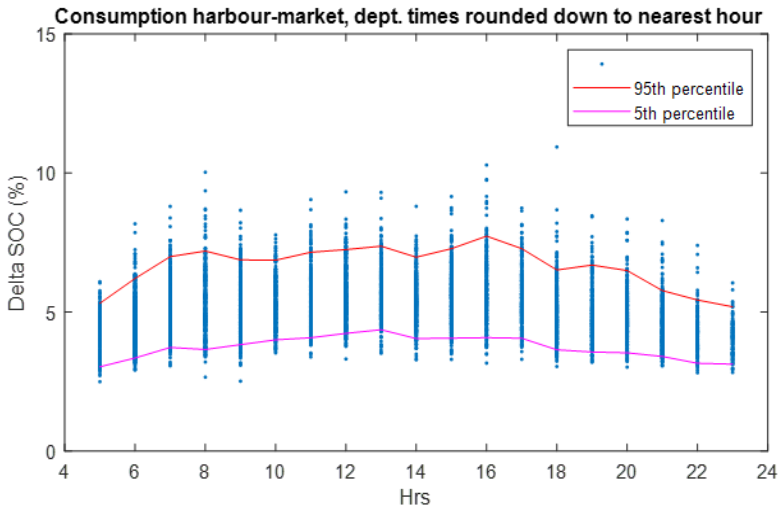
Figure 23. Delta soc vs. the departure time.
