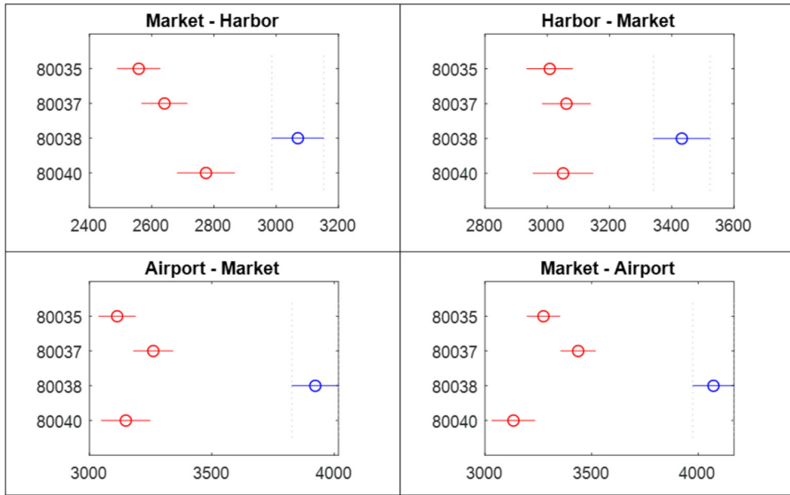
Figure 22. The results from a non-parametric statistical test indicate that vehicle 80038 consumes more energy than the other vehicles on a statistically significant level ( \alpha = 0.05 )
