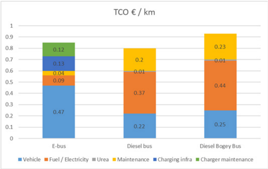
Figure 35. TCO analysis of an e-bus system compared to various types of diesel buses (Lankila 2017)
