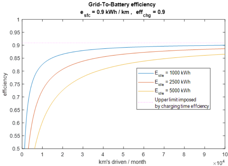
Figure 17. System level efficiency with varying levels of idle consumption.
