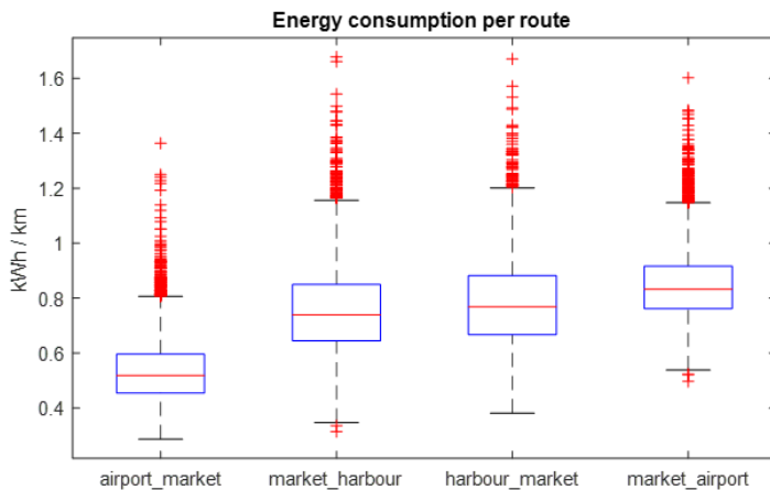
Figure 20. Distribution of energy consumption (kWh / km) approximated from Delta SOC. For illustrative purposes only.
