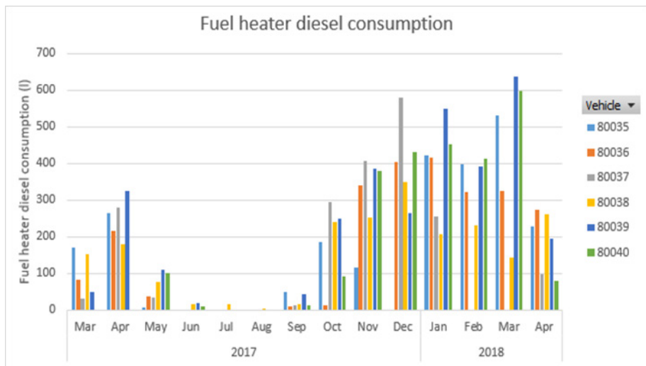
Figure 18. Fuel heater diesel consumption by month and vehicle
