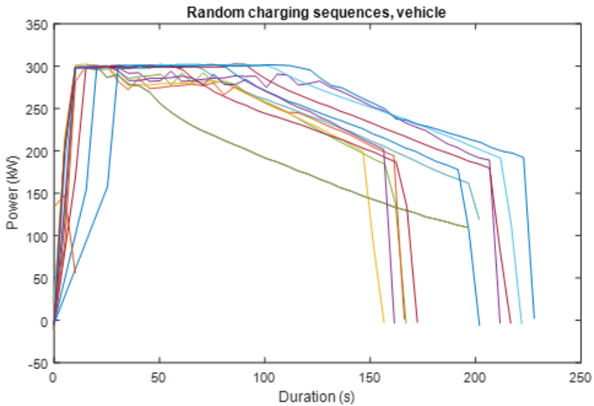
Figure 33. Random charging sequences measured from vehicle
