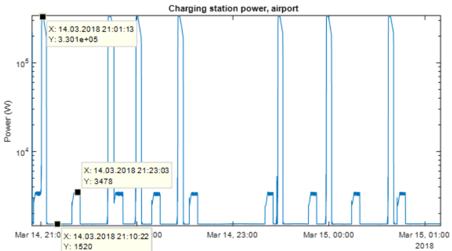
Figure 31. An excerpt of the charging station power measurements
