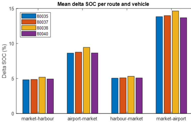
Figure 21. Mean energy consumption (delta soc %) by route segment and vehicle.
