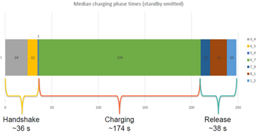
Figure 13. The median durations of the different phases in the fast charging events (N = 2385) as recorded by vehicle 80035 during 10/16 – 03/17
