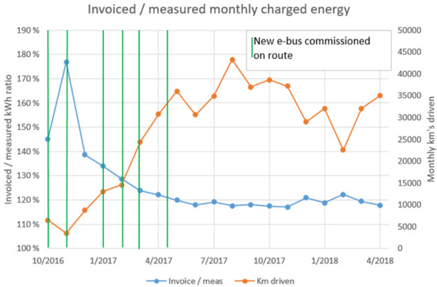
Figure 15. Invoiced and measured monthly charged energy and monthly kilometers
