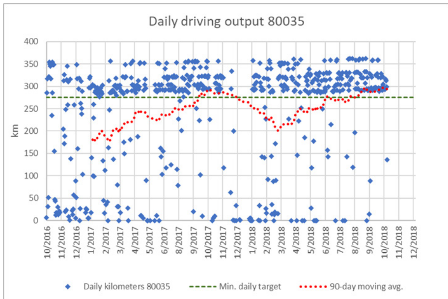
Figure 10. The realized driven kilometers from a single vehicle October 2016 – November 2018
