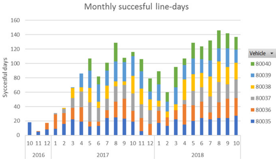
Figure 12. Classification of days according to kilometers driven, aggregation by month and vehicle
