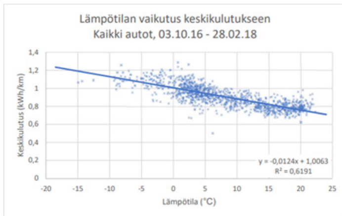
Figure 28. Average daily consumption (kWh / km) vs. average daily temperature (° C) (Taavetinkangas 2018)
