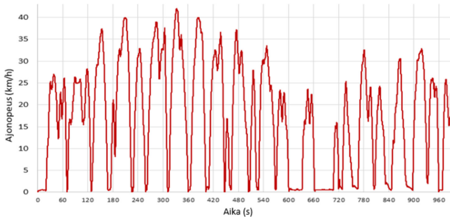
Figure 5. An excerpt of the velocity graph representative of bus operation on route 1 (Turun Kaupunki 2016)
