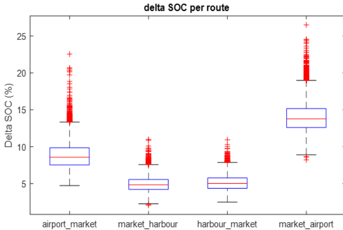
Figure 19. Distribution of energy consumption (Delta SOC) on different route segments
