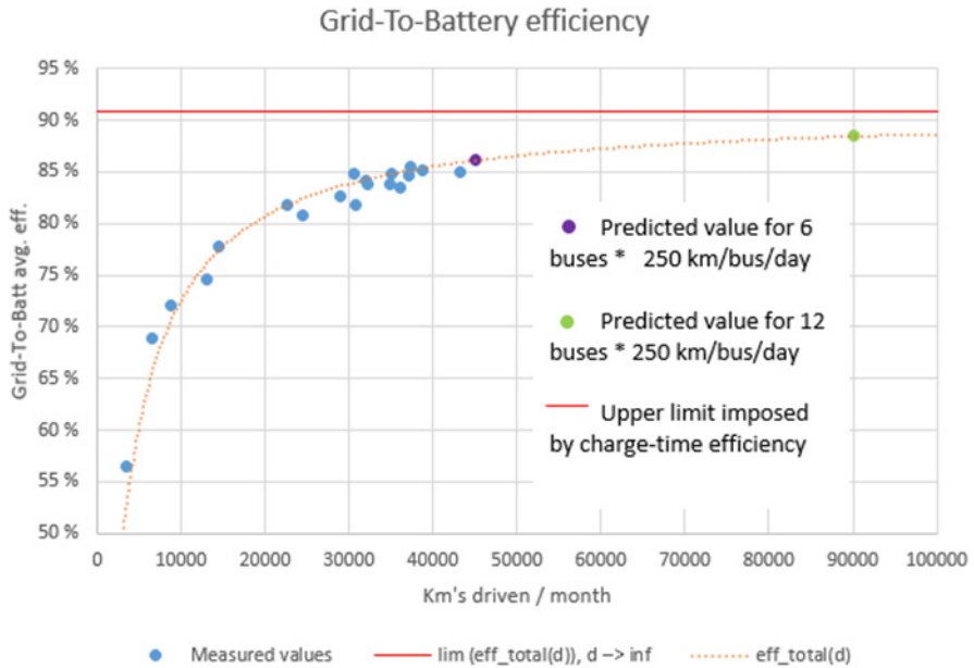
Figure 16. Modelling the grid-to-battery efficiency as a function of monthly driven kilometers with constants: e_{sfc}=0.9 kWh/km , eff_{chg}=0.9 , E_{idle}=2500 kWh .
