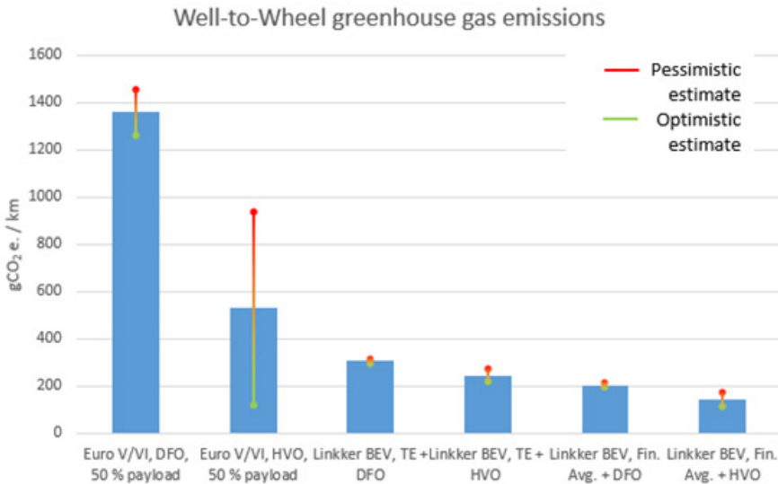
Figure 39. Well-to-Wheel analysis of various fuels of transportation. Linkker values include the operation of fuel heater.
