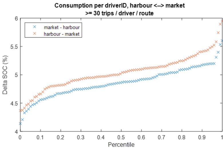
Figure 25. Average delta SOC for driverID, Harbor - Market
