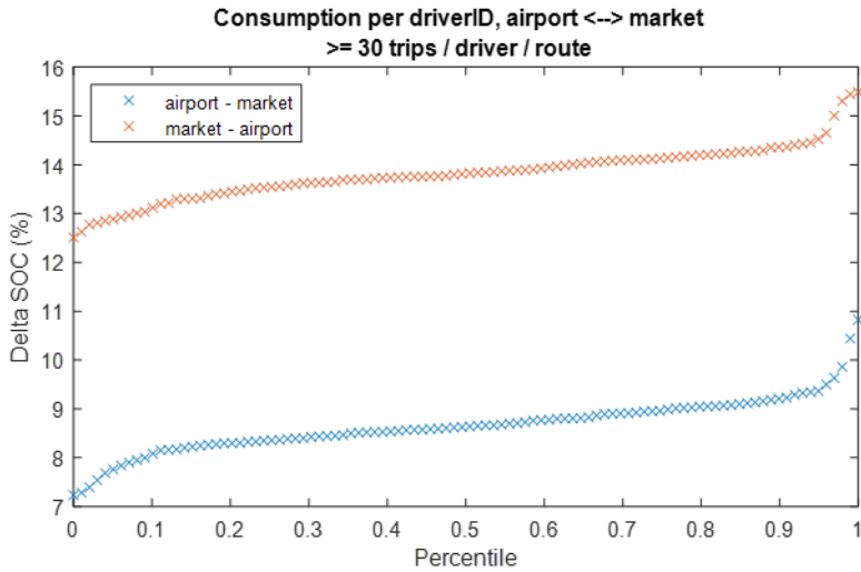
Figure 24. Average delta SOC for driverID, Airport - Market
