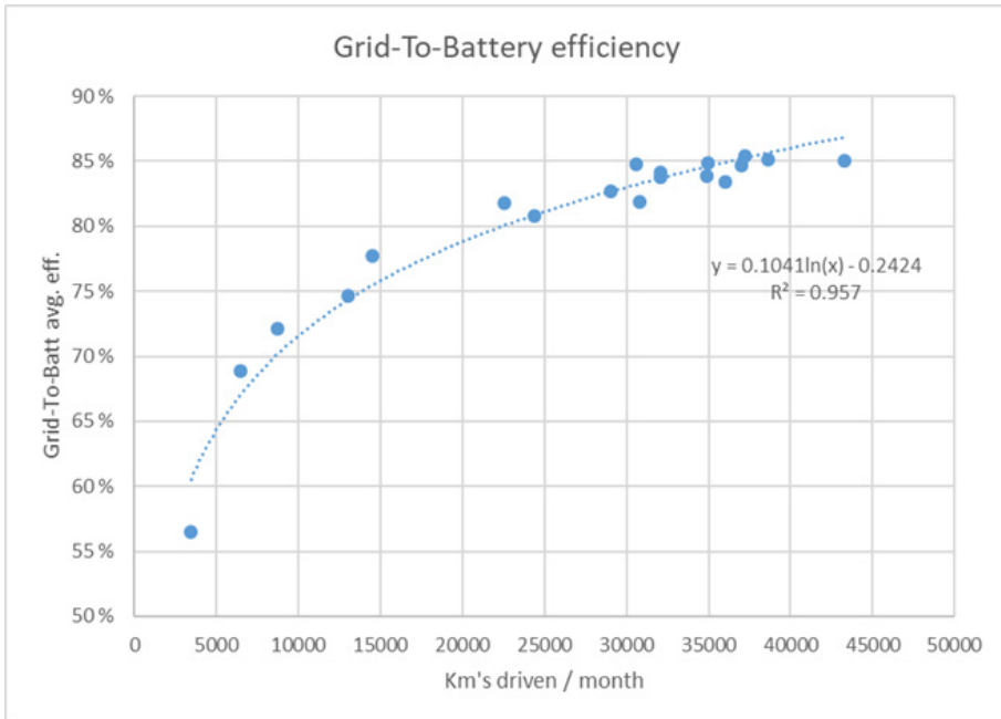
Figure 14. Grid-to-battery average efficiency as a function of monthly kilometers. We provide a logarithmic fit for visualization purposes only.
