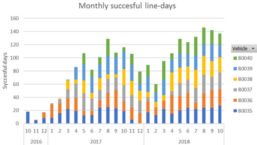
Figure 2. Classification of days according to kilometers driven, aggregation by month and vehicle
