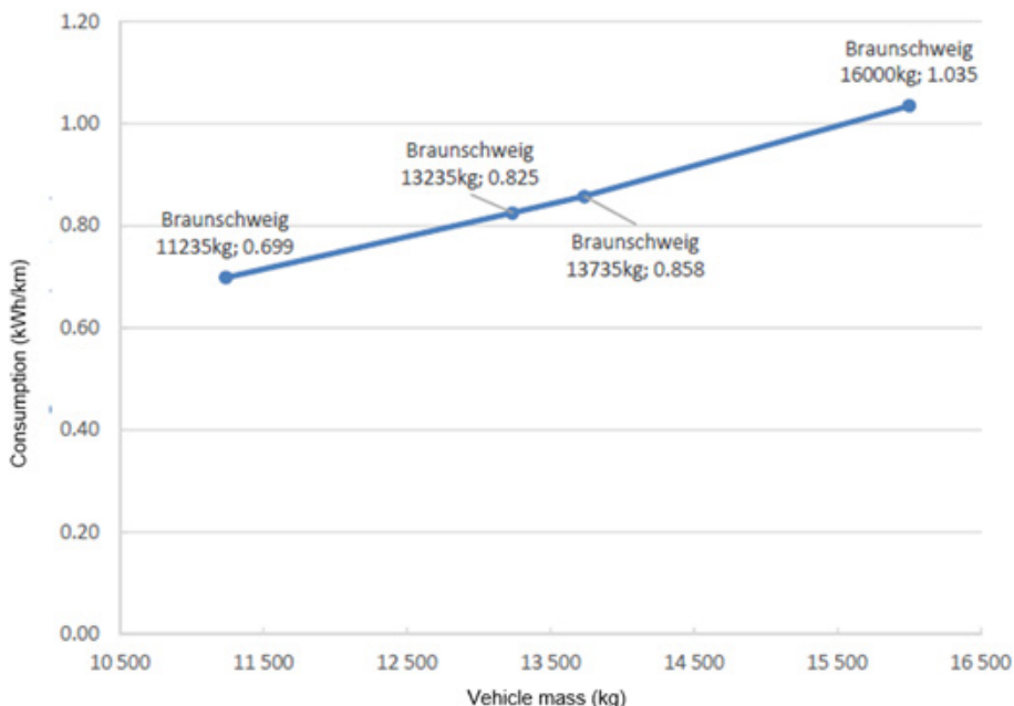
Figure 34. The effect of payload on consumption (Anttila 2017)
