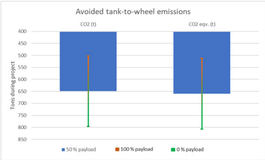
Figure 37. Avoided tank-to-wheel GHG emissions during the project’s pilot phase
