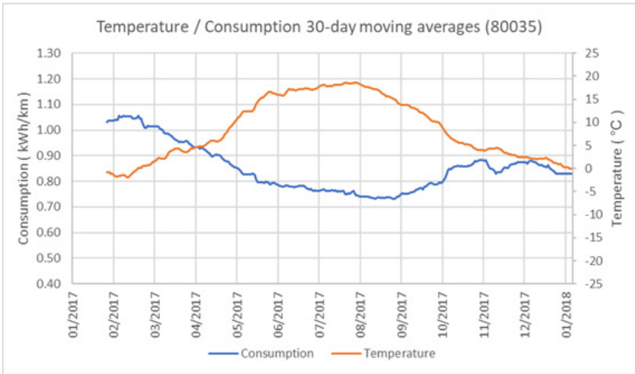
Figure 26. Seasonal trend in energy consumption
