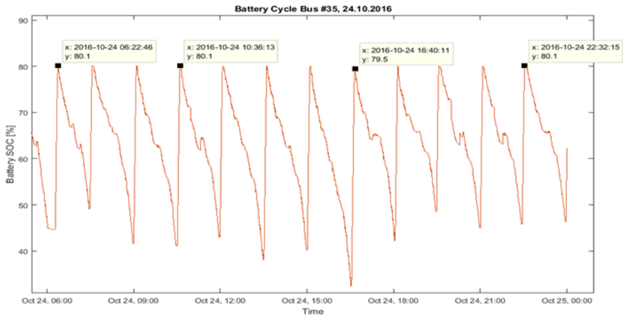
Figure 7. During normal operation, the battery State of Charge (SOC) mostly remains between 40 % - 80 %, which is known to be beneficial for the battery lifetime.
