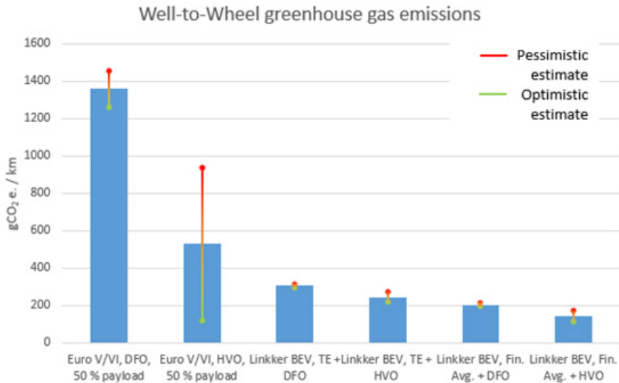
Figure 3. Well-to-Wheel analysis of various fuels of transportation. Linkker values include the operation of fuel heater.
