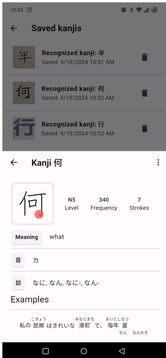
Figure 29. The user can bookmark kanjis and look at them later
