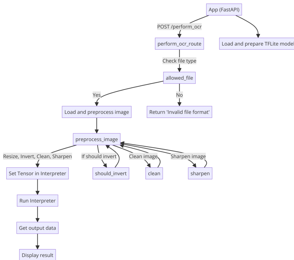
Figure 26. Modified backend flowchart that uses TFLite on the Render cloud
