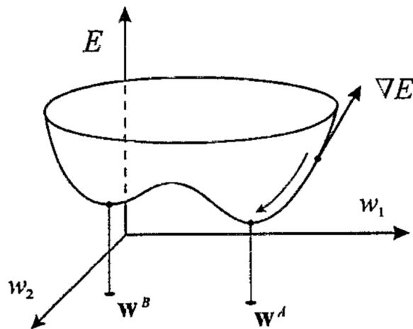
Figure 16. The cost function E(w) seen as a surface over weight space (the space spanned by the values of the weight and bias parameters w = \{w_1, \dots, w_L\} ) (Bishop, C. M. 1994).
