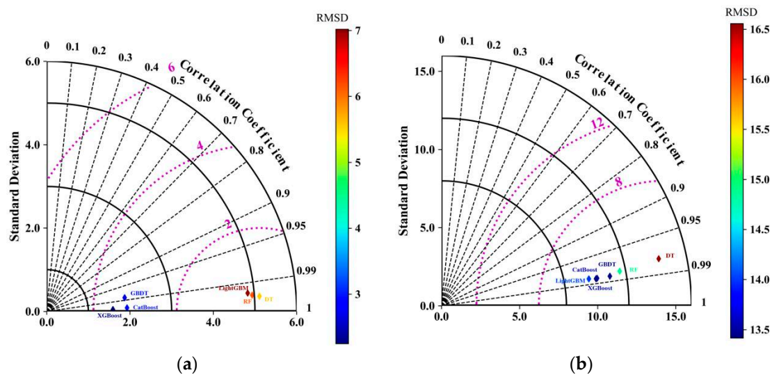
Figure 8. Performance of each machine learning model.
