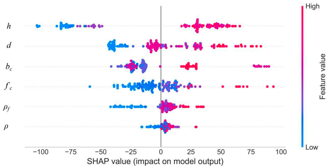
Figure 9. SHAP summary plot.
