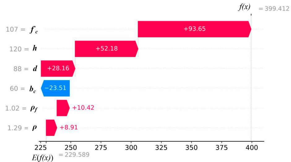
Figure 10. SHAP waterfall plot.
