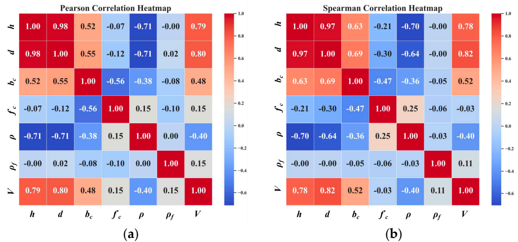
Figure 2. Correlation coefficients of parameters. (a) Pearson’s correlation coefficient; (b) Spearman’s correlation coefficient.
