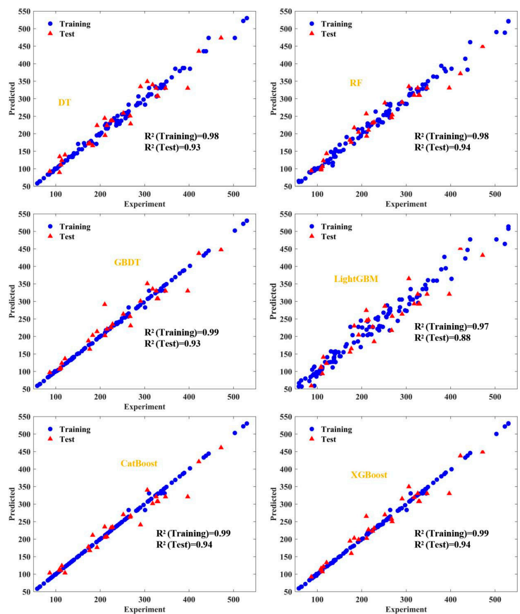
Figure 4. Predicted vs. real values under M1.
