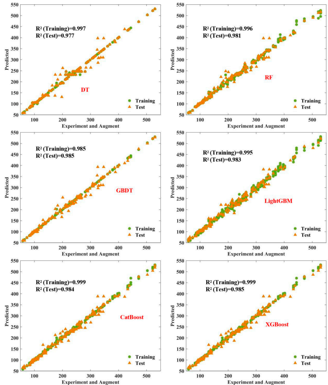
Figure 5. Predicted vs. real values under M2.
