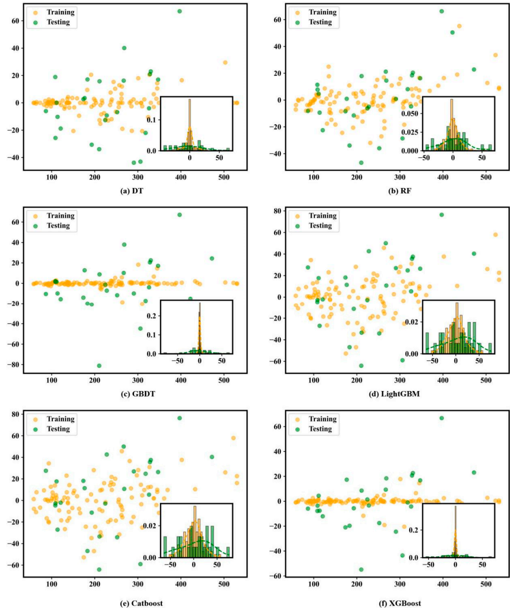
(A) Distribution of deviations under M1
