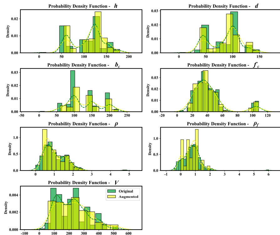
Figure 3. Data distribution before and after augmentation.
