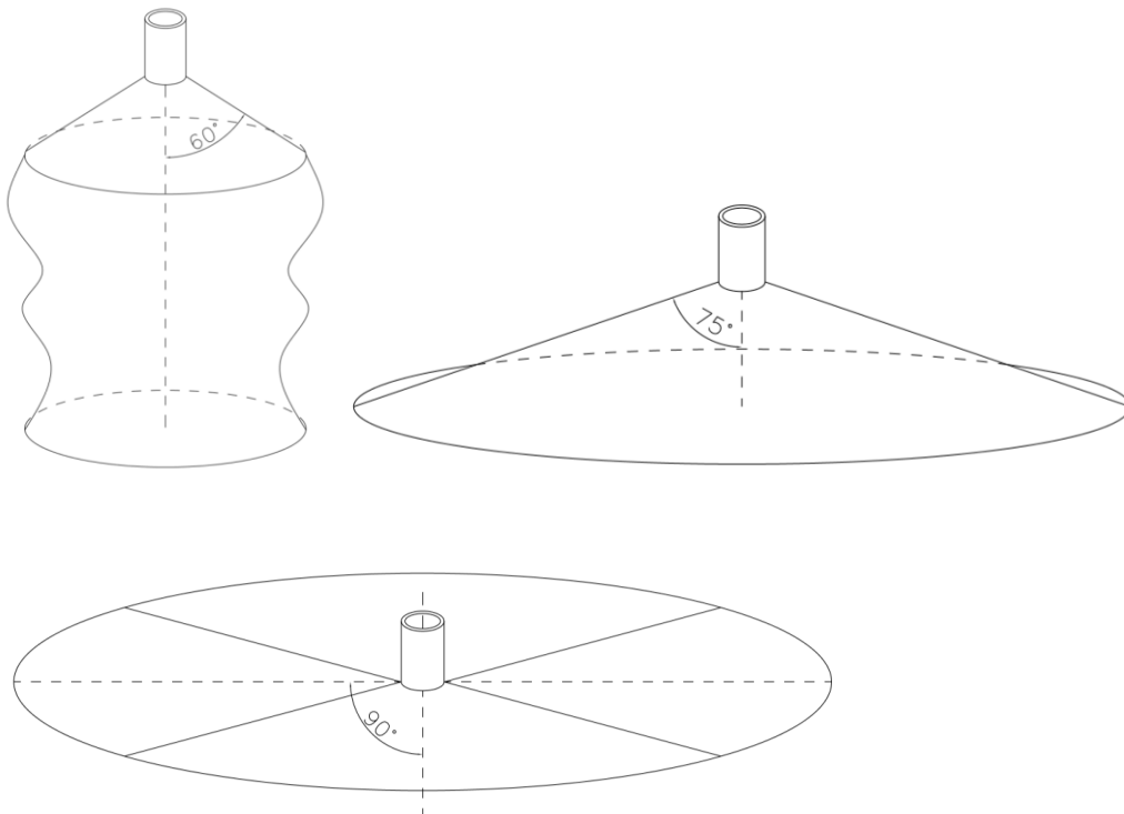
Figure 5.21. Conical air jets
