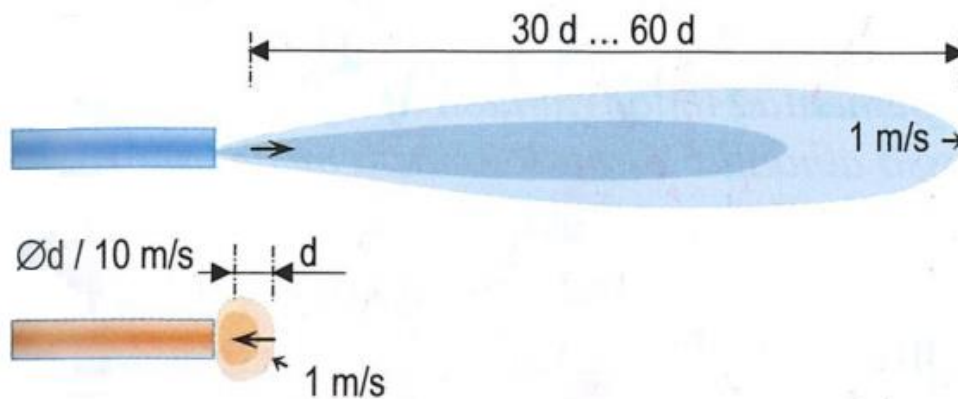
Figure 5.14. Difference between supply air and extract air streams (Sandberg, 2014)
