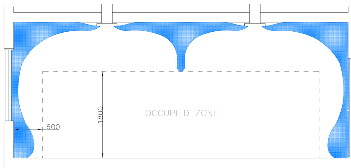
Figure 3.6. Occupied zone and air streams
