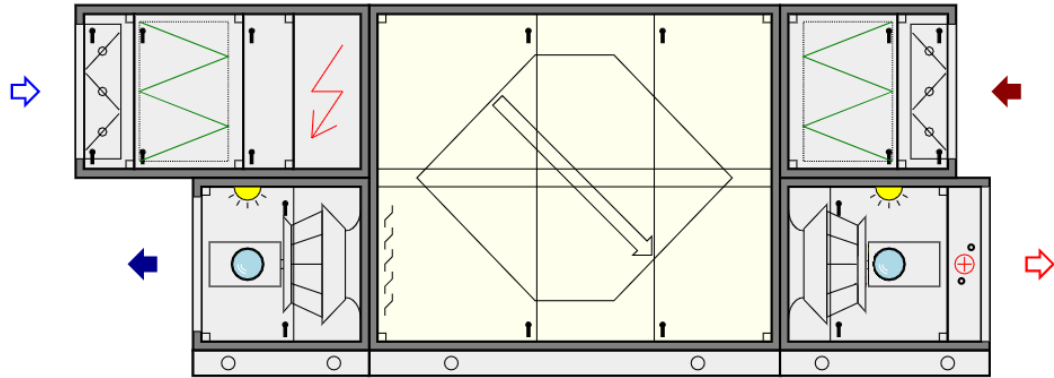
Figure 5.6. Air handling unit with preheating coil and counter flow heat exchanger (FläktWoods Acon, Air handling unit selection program)
