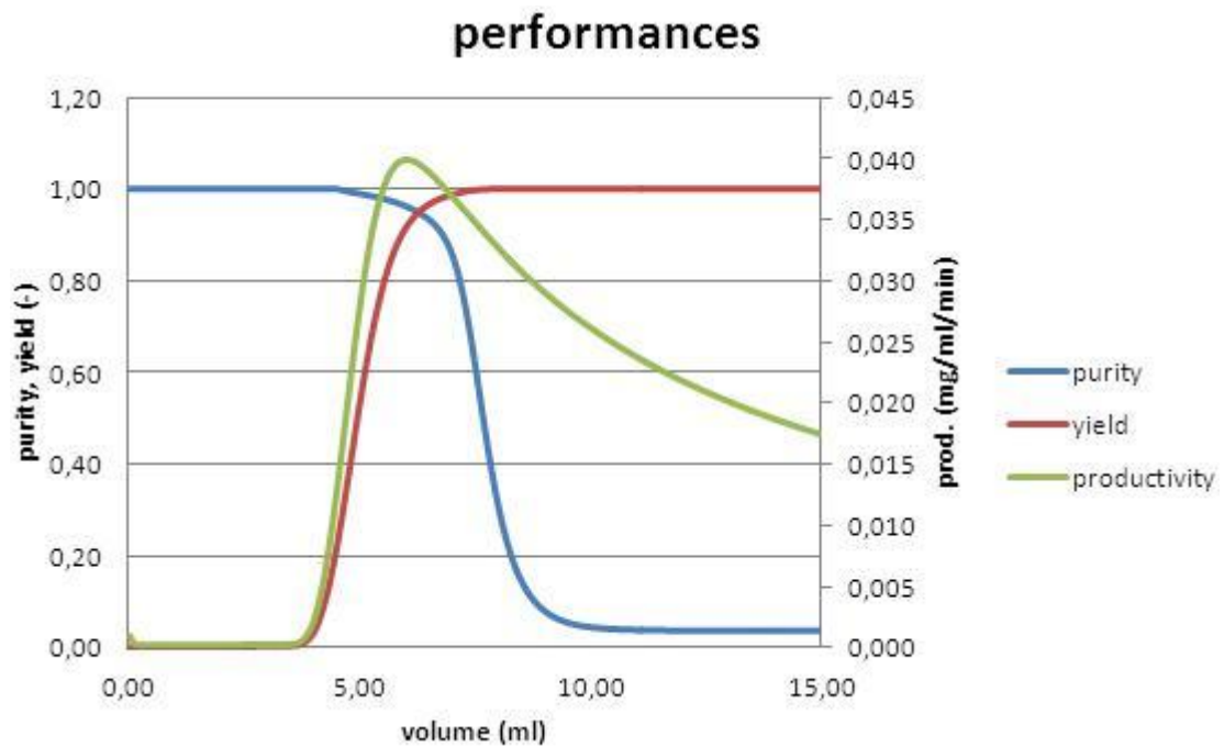
FIGURE 14. Chromatography performances
