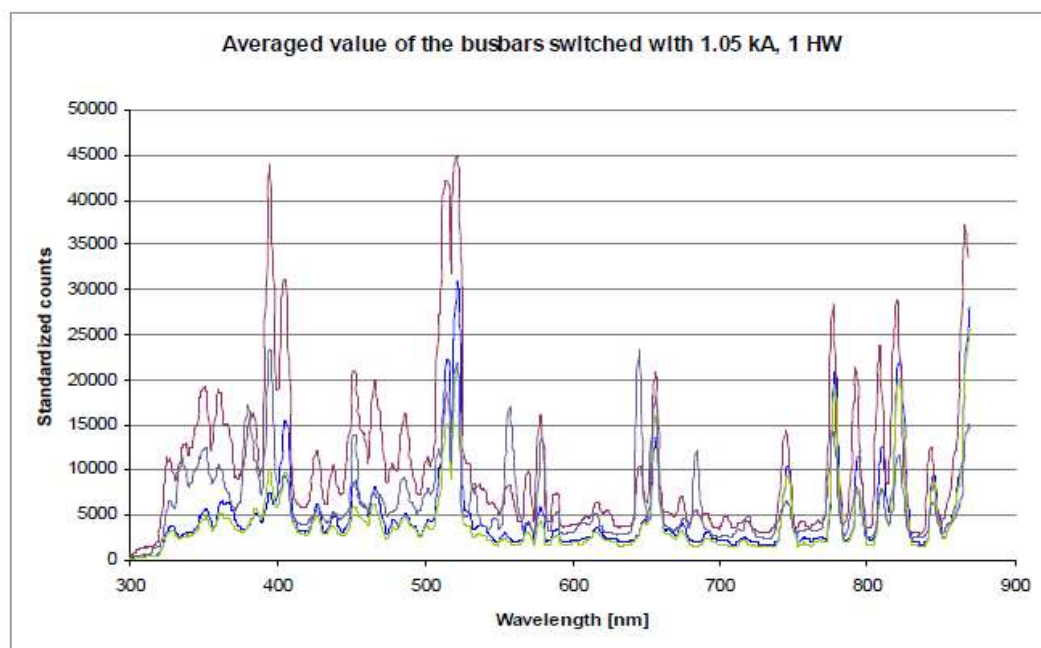
Figure 9. Measurement result from of arc light spectrum distribution.[2]
