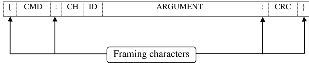
Figure 23. Serial communication, response message structure
