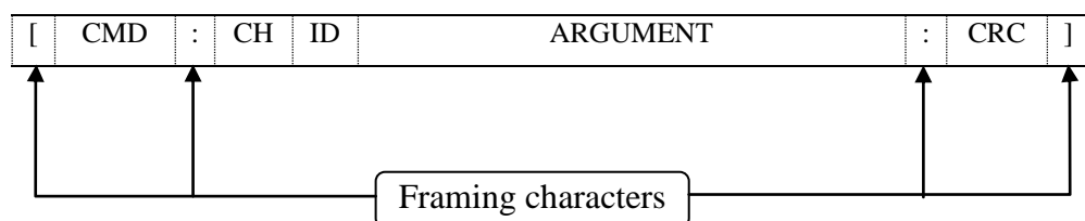
Figure 22. External Serial communication, request message structure
