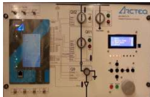
Figure 5. AQ-SIM F215 simulator
