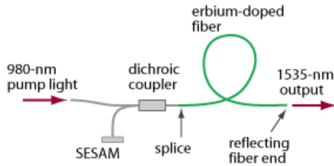
Figure 5.9 Simple Q-switch fiber laser schematic diagrams (Rp)
