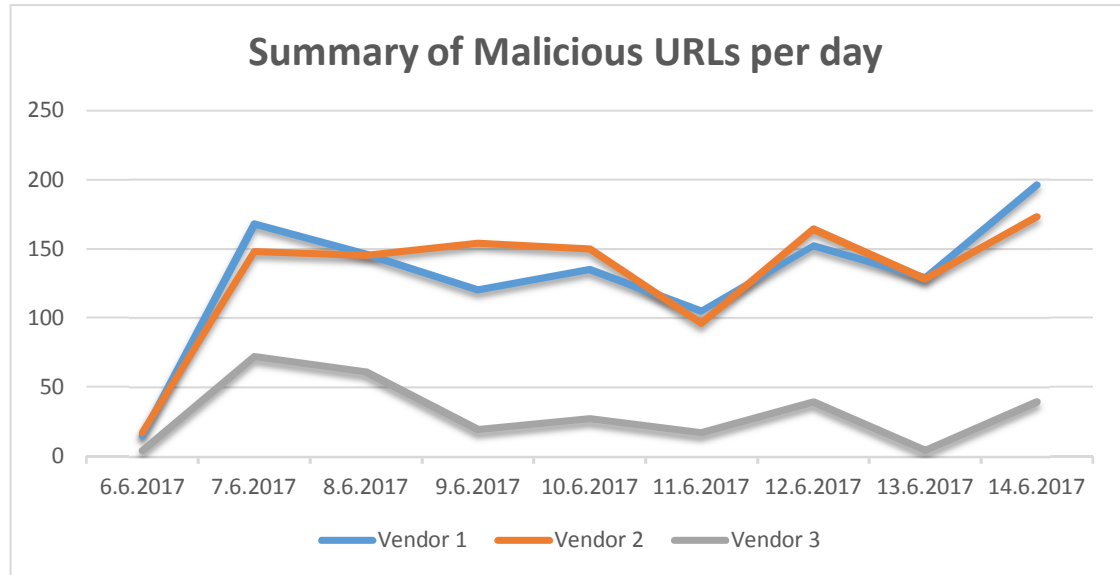
Figure 14. Summary of Malicious URLs per day
