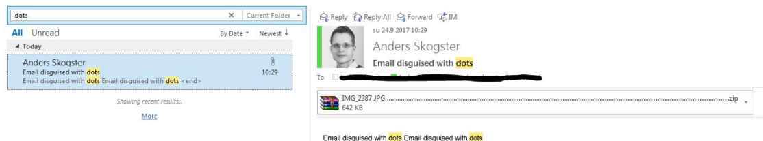
Figure 7. Attachment disguised with dots – Outlook
