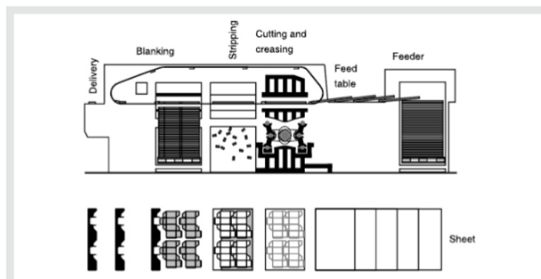
Figure 6. Flat bed cutting and creasing machine 1,18 .
