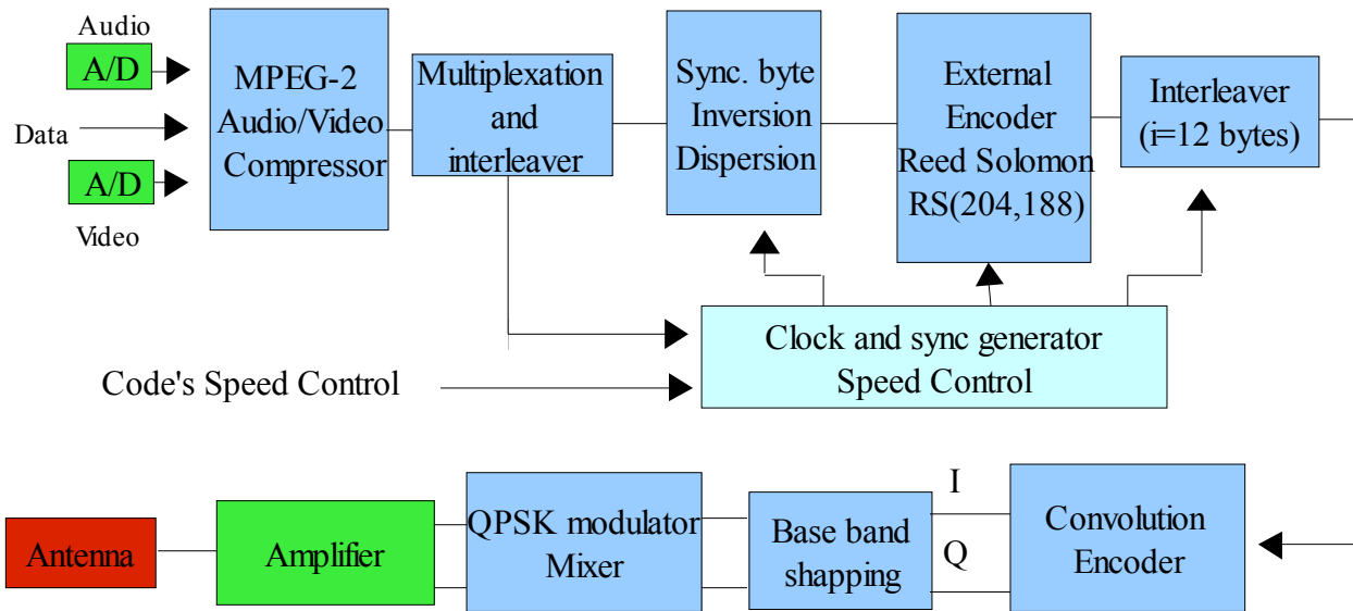
Fig.3 Block of DVB-S standard transmission
