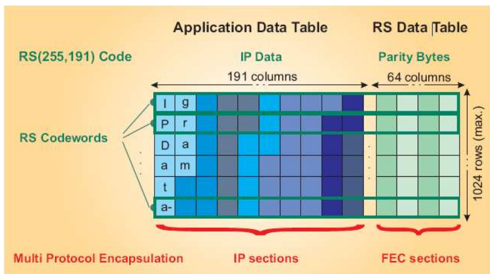
Fig. 11: MPE-FEC structure
