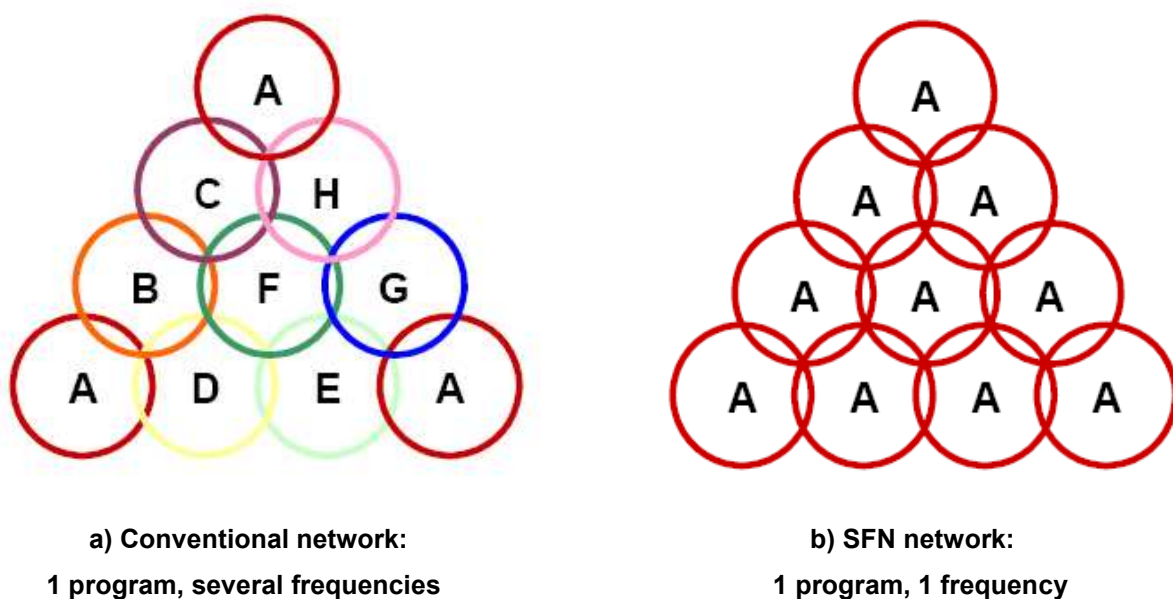
Fig. 9 Radiowaves planning
