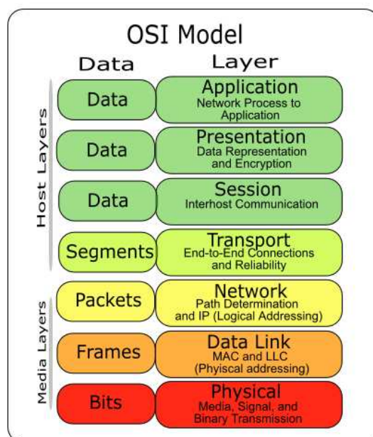
Fig.8 OSI model
