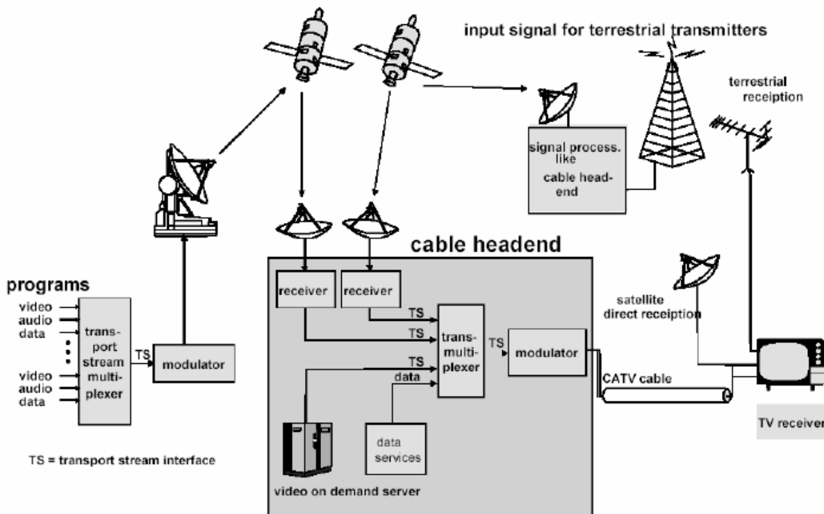
Fig.2 Scheme of standards DVB-T,DVB-S,DVB-C application
