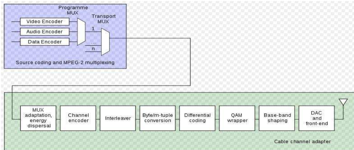
Fig.5: Blocks diagram of DVB-C transmission
