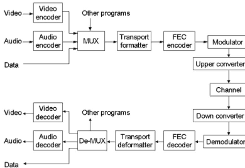
Fig.6: Block diagram of DVB-T standard
