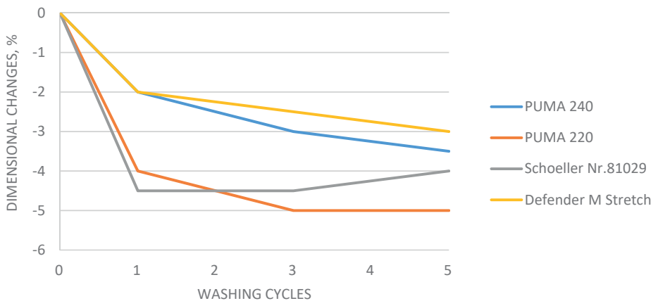
Figure 1.3. Dimensional changes after washing and drying at 60°C
