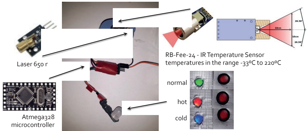
Figure 7.26. The unit for remote surface temperature control
