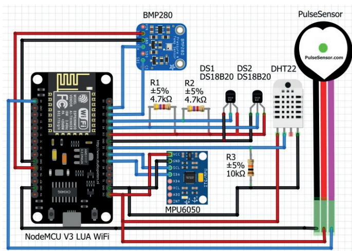
Figure 7.18. Smart vest controllers assembly scheme
