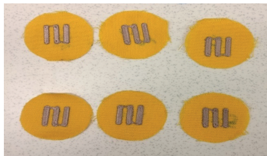
Figure 6.8. Cut sample of copper PLA on fabric F1, each sample have diameter of 30mm.
