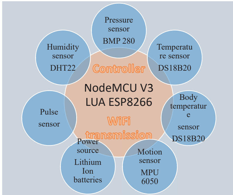
Figure 7.17. Electronic scheme of smart vest
