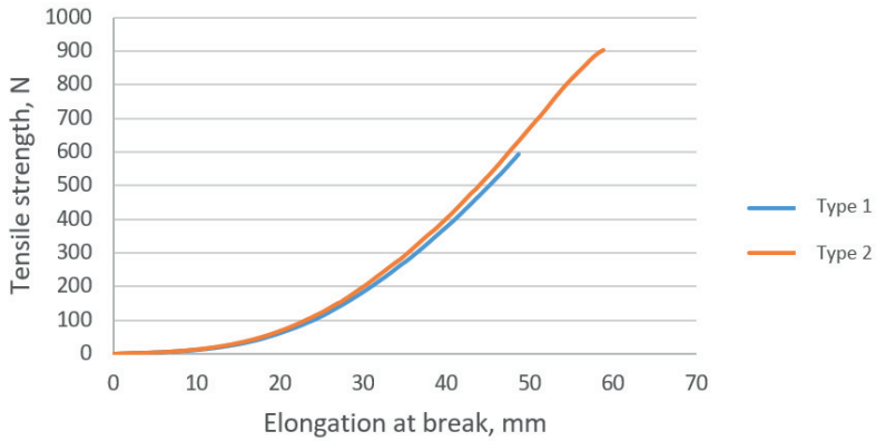
Figure 1.12. Seam strength for PUMA 220 joint lengthwise
