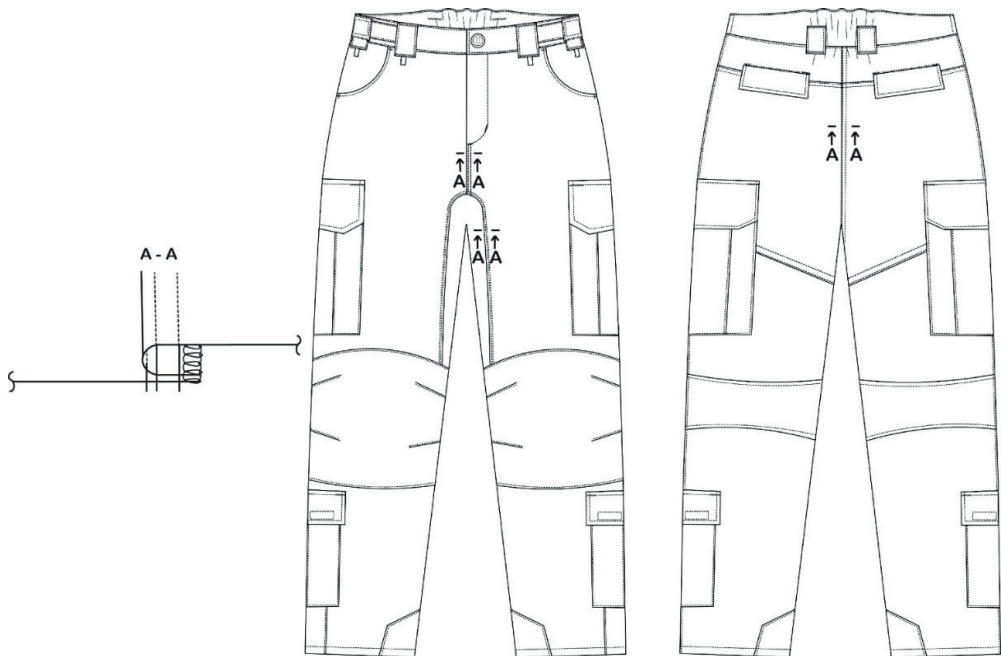
Figure 1.16. Technological drawing of trousers
