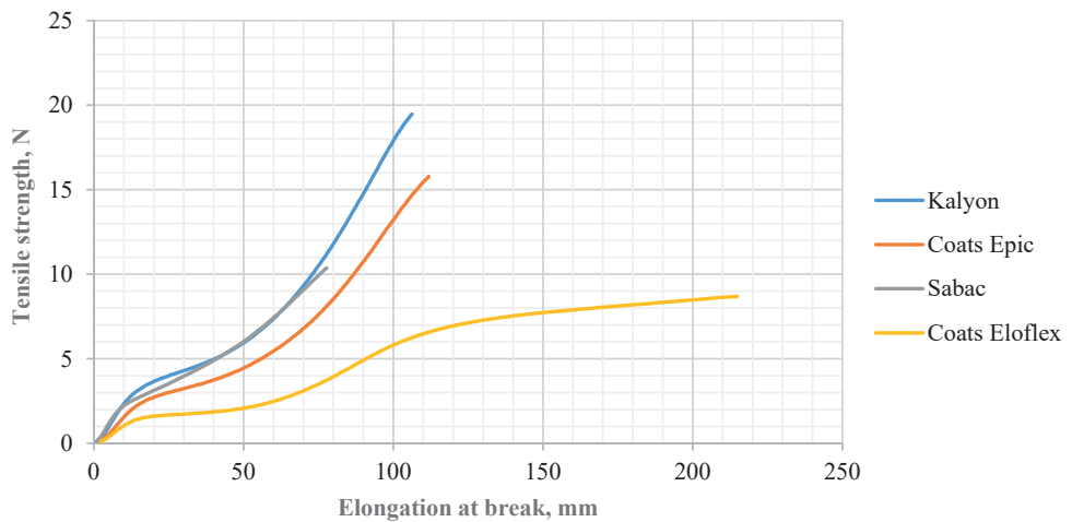
Figure 1.9. Tensile strength of sewing threads
