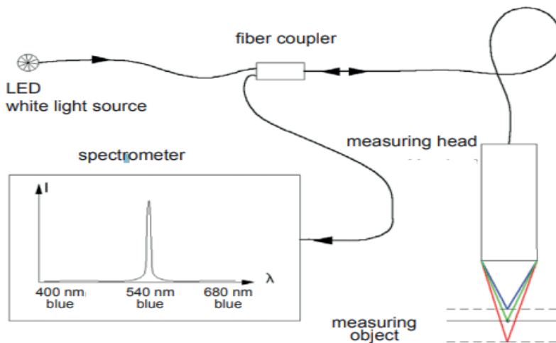
Figure 6.18. Surface roughness measurement set up
