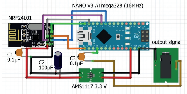
Figure 7.12. Transmitters assembly scheme
