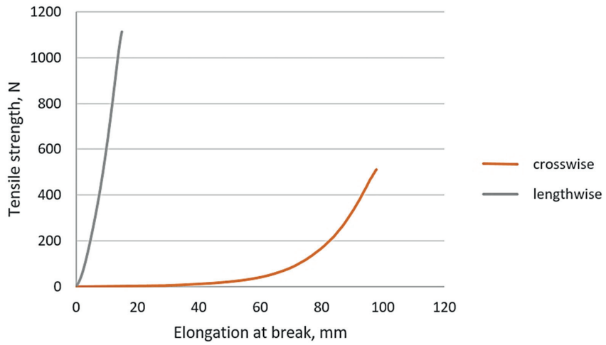
Figure 1.8. Tensile strength of Defender M Stretch
