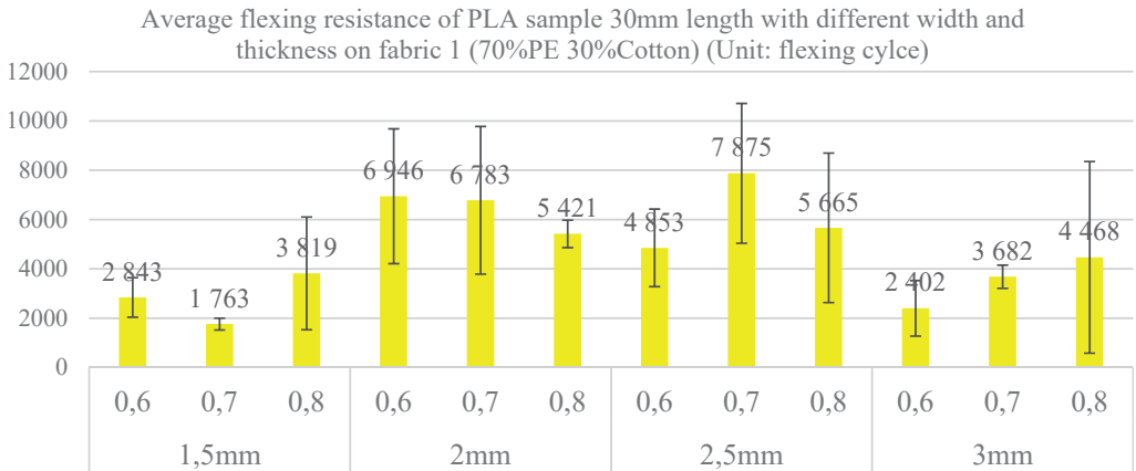
Figure 6.6. Average flexing resistance of PLA sample
