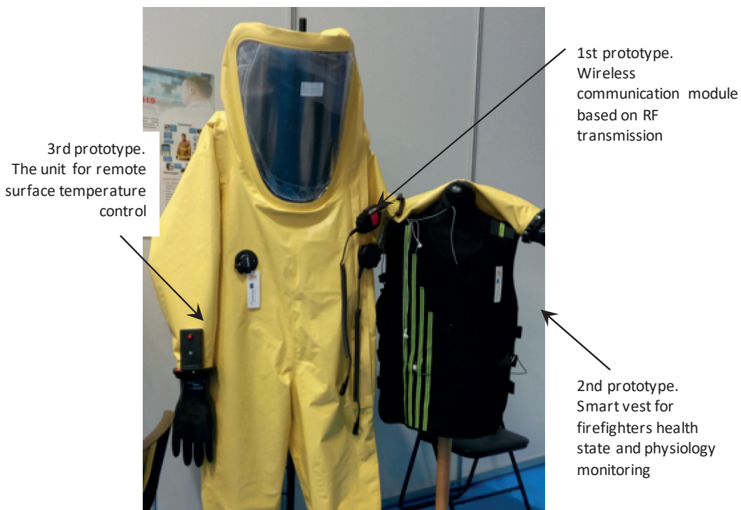
Figure 7.25. Three prototypes of safe CPC suit
