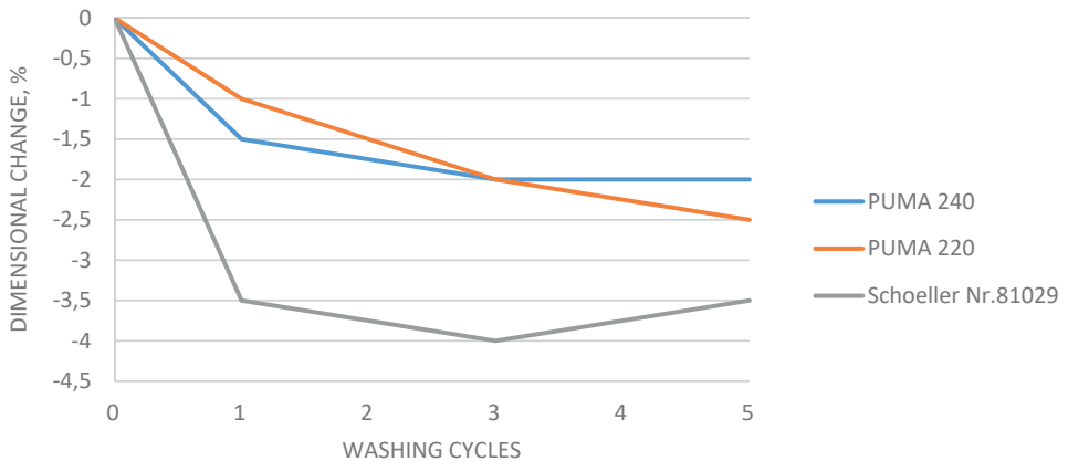
Figure 1.1. Dimensional changes lengthwise after washing at 60°C
