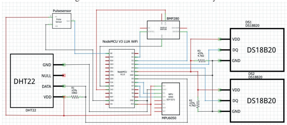
Figure 7.18. Smart vest controllers assembly scheme
