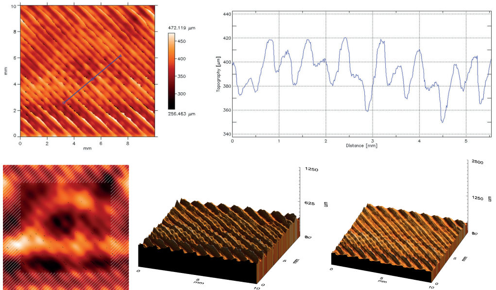
Figure 6.20. Analysis of 3D microscopic image (standard PLA)
