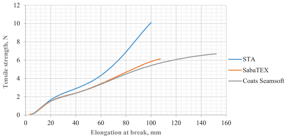
Figure 1.10. Tensile strength of overseaming threads
