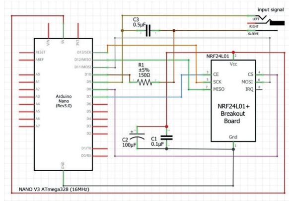
Figure 7.15. Principal electronic diagram of receiver
