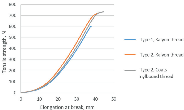
Figure 1.11. Seam strength for the PUMA 220 joining crosswise
