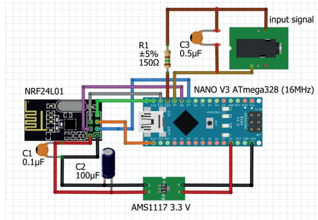
Figure 7.14. Receiver assembly scheme
