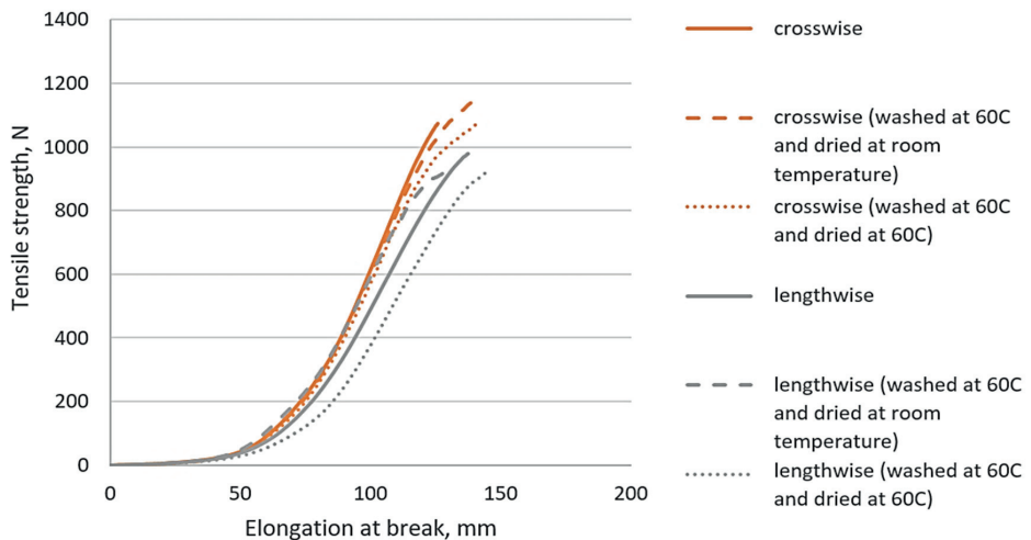
Figure 1.7. Tensile strength of Schoeller No 81029
