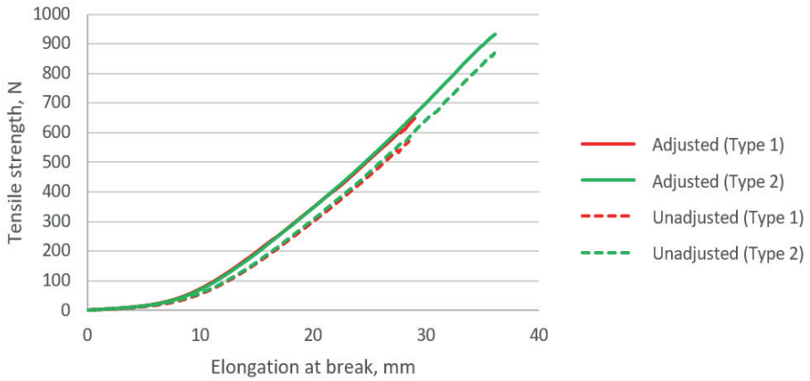
Figure 1.15. Tensile strength depending on thread tension
