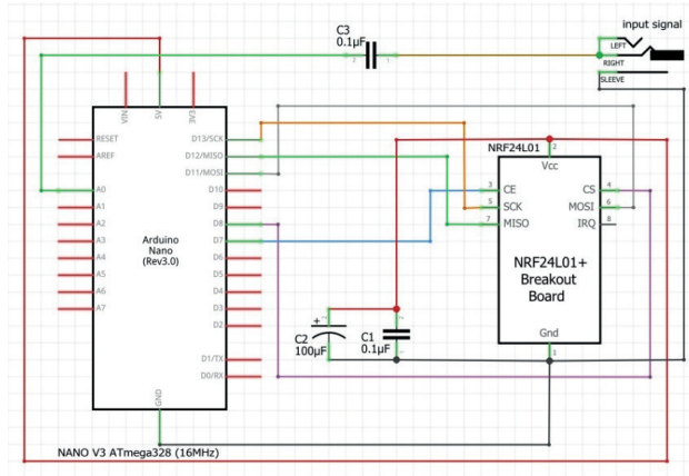
Figure 7.13. Principal electronic diagram of transmitter
