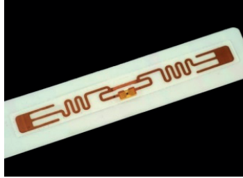
Figure 4.6. Solution using metallic conductive paints [82]
