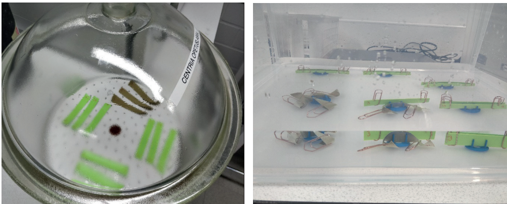
Figure 6.21. Water absorption testing of 3D printed samples
