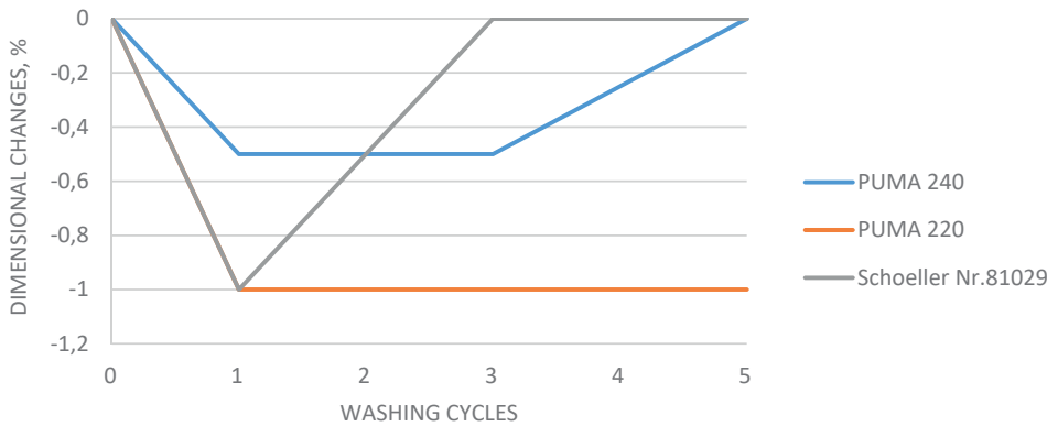
Figure 1.2. Dimensional changes crosswise at 60°C
