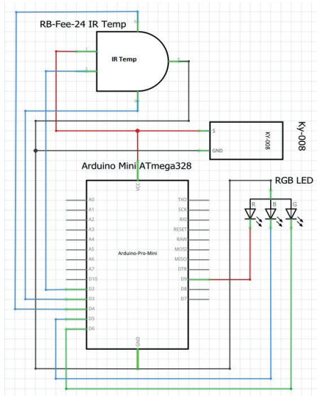
Figure 7.28. Principal electronic diagram of remote surface temperature control unit
