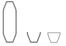
BLADE FOR CAST AIR NOZZLE 600cm2 P63.5 R95 J78 C02STDDR026_1110112_4651121
