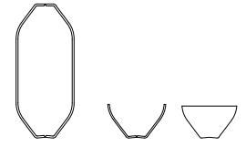
BLADE FOR CAST AIR NOZZLE 800m2 P63.5 R95 J84 C02STDDR026_1110112_4807121
