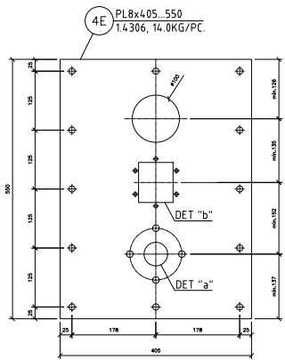
RODDER FASTENING PLATE 4
