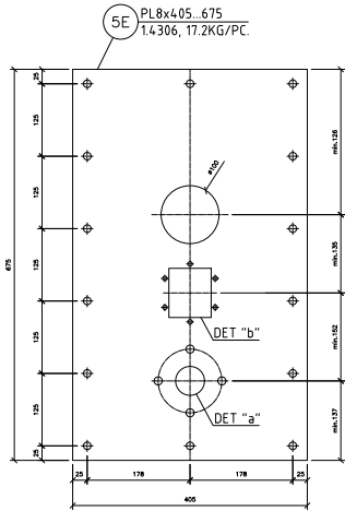
RODDER FASTENING PLATE 5
