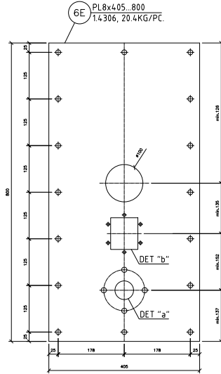
RODDER FASTENING PLATE 6
