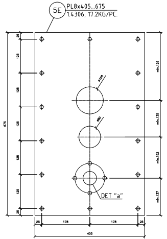
RODDER FASTENING PLATE 5
