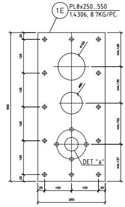
RODDER FASTENING PLATE 1
