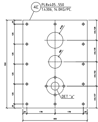
RODDER FASTENING PLATE 4
