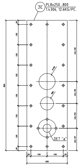
RODDER FASTENING PLATE 3
