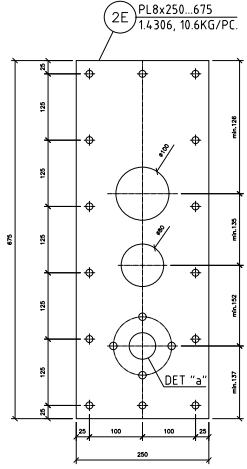
RODDER FASTENING PLATE 2
