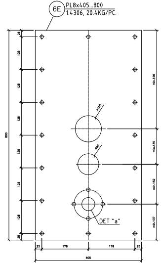
RODDER FASTENING PLATE 6
