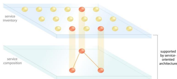
Fig. 5 Service composition in SOA [12]
