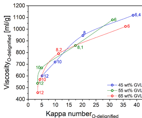
Fig. 2. Pulping selectivity of oxygen-delignified pulps for the cooks with L: W = 10 at different GVL concentrations. The digits in the graph represent the H 2 SO 4 concentration in kg/t (more details in Table S1).
